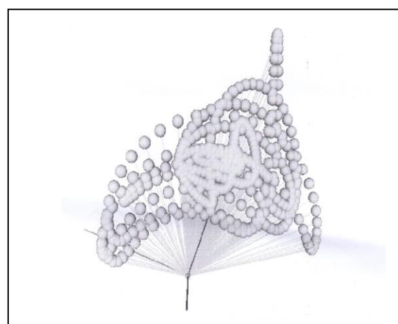
Figure 3 - Three-dimensional structure of blood Albumin (585 Amino Acids)
