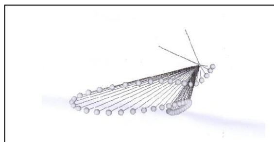
Figure 2 - Three-dimensional structure of human Insulin (51 Amino Acids: 21 in subunit A and 30 in subunit B)
